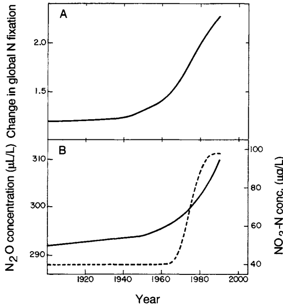
FIG. 9. Changes in global N fluxes during the 20th century. (A) Human alteration of global N fixation as the ratio of anthropogenic to total (anthropogenic plus natural) N fixation (from Fig. 8). (B) Concurrent patterns in atmospheric concentrations of the greenhouse gas nitrous oxide (—) (Watson et al. 1990) and in nitrate concentrations at the mouth of the Mississippi River (---) (Turner and Rabelais 1991).
