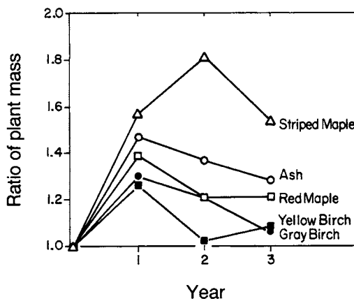
FIG. 6. The time course of growth enhancement caused by elevated \text{CO}_2 concentration for several New England tree species. The response ratio is calculated as growth of a given species at 680 \mu\text{L/L CO}_2 divided by its growth at 340 \mu\text{L/L CO}_2 . All of the species initially respond positively, but they differ substantially in how long elevated growth rates are maintained. From Bazzaz et al. (1994); reproduced with permission.
