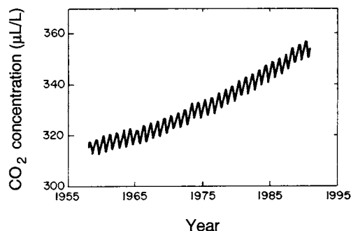
FIG. 2. Measured concentrations of \text{CO}_2 in the atmosphere at Mauna Loa, Hawaii. The annual cycle is driven by seasonal activity of terrestrial biota in the northern hemisphere, while the overall increase is driven primarily by fossil fuel combustion (Keeling et al. 1989a, b). From data in Keeling and Whorf (1991).
